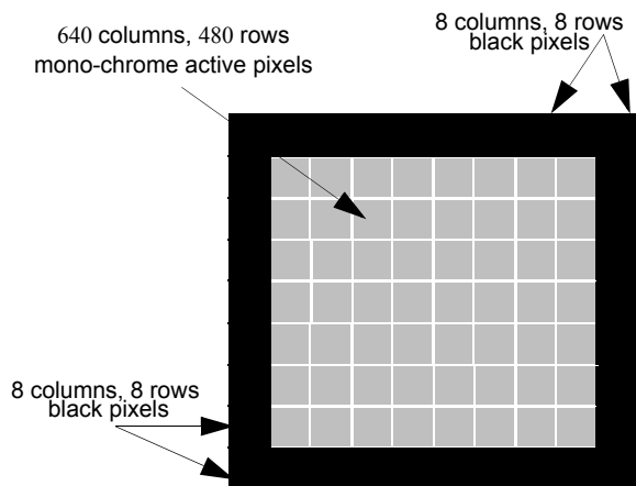
Figure 7: CMOS APS region of the KAC-9619
