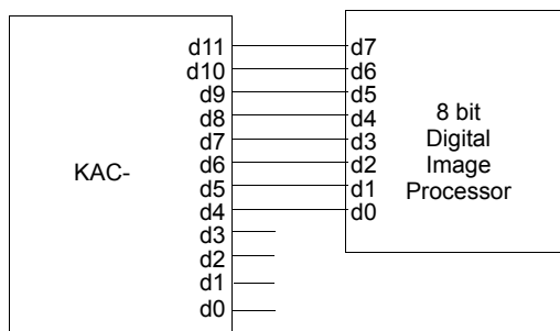
b) KAC-9619 Connected to a 8 bit Digital Image Processors
