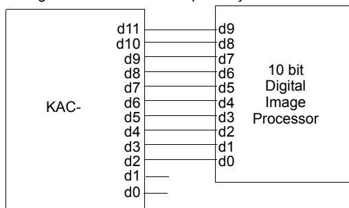
a) KAC-9619 Connected to a 10 bit Digital Image Processors
