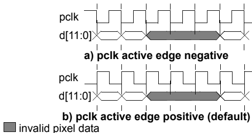
Figure 37. pclk in Free Running Mode
