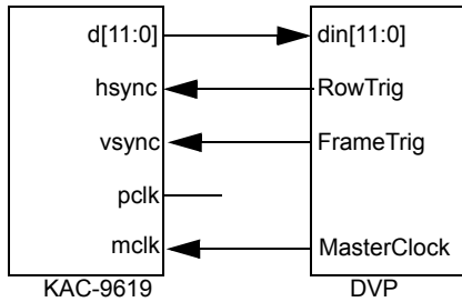
Figure 48. KAC-9619 in slave mode
